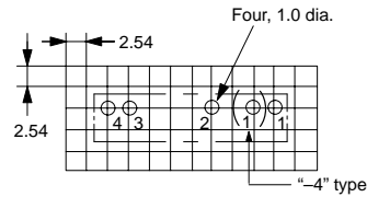
PCB Dimensions (Bottom View)
